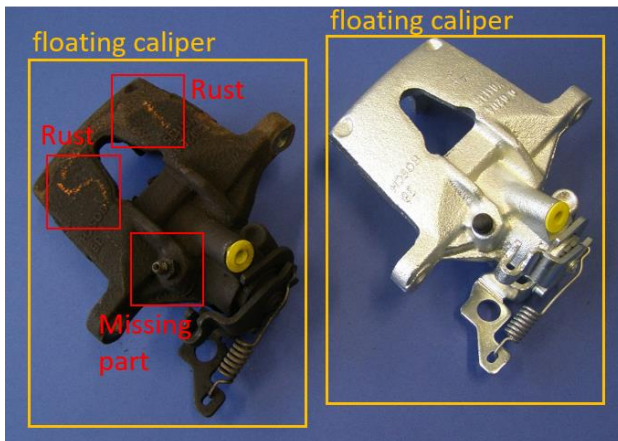
"Turn old into new": old part and refurbished part, ready for a second life in the vehicle.
