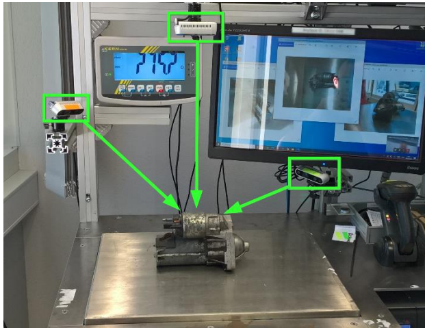
Prototype workstation with sensor equipment in EIBA project
