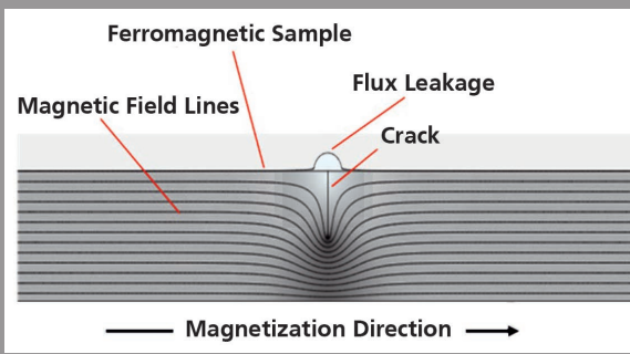
1: Magnetic flux leakage – principle
