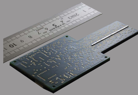
2: Linear array of highly sensitive magnetic field sensors
