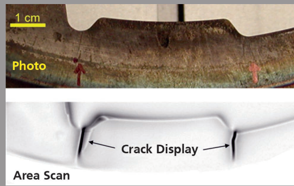
3: Crack visualization after induction hardening
