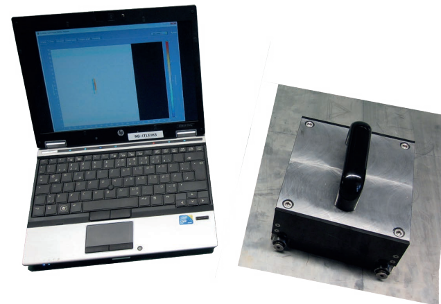
5: FLUXI in use on sheet steel with test defect
