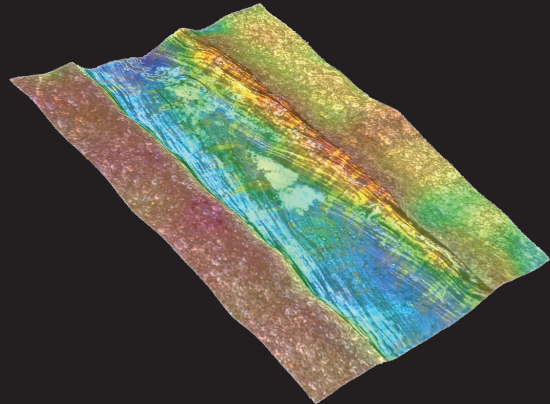
3d profile of a laser beam welding seam
